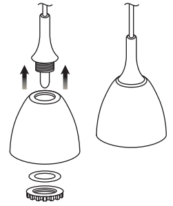
Lock-Fit Assembly
