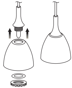
Lock-Fit Assembly
