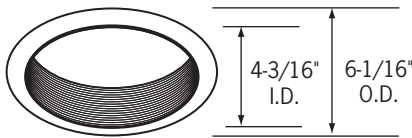
CTR4321V-B Black Baffle, Clear Specular Reflector, Black Metal Trim Ring
