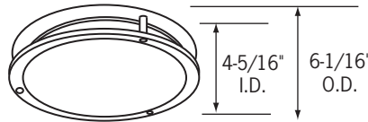
CTR4325V-P Floating Glass Trim White specular reflector supported by (3) chrome posts, 1-1/4" drop from ceiling.
