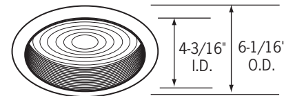
CTR4327V-P Black Baffle Trim
