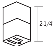
LA-1B 15/16" Grid Deep Tile T-Bar Clip. Fits into channel in back of track. May be spaced to 4'. Finish: -S
